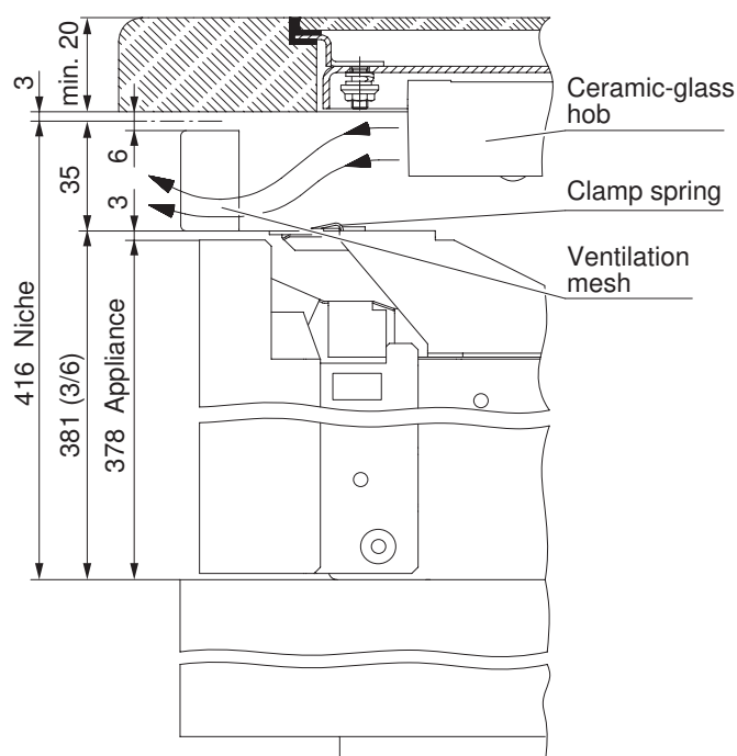
View A Oven 55-381, 60-381
