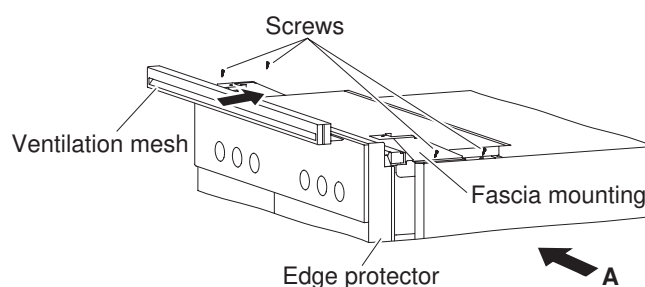
View A Oven 55-381, 60-381
