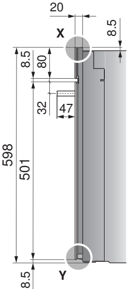
Appliance without drawer
