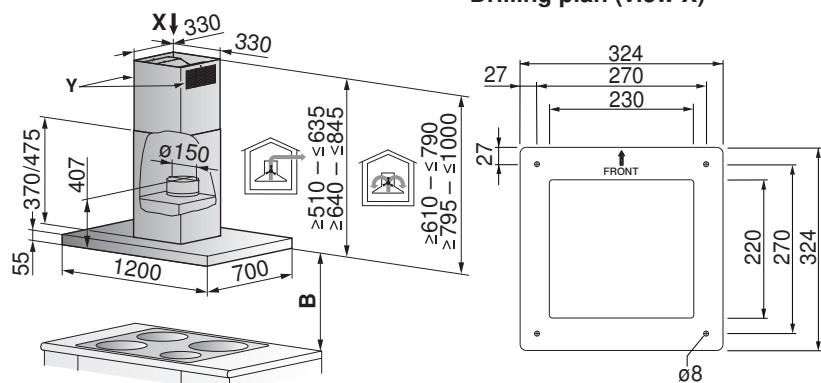
Drilling plan (view X)
