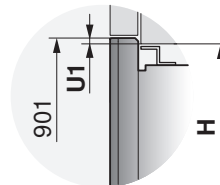
Detail X
