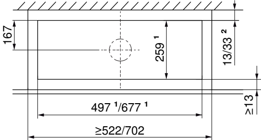
Cut-out for wall unit (view X)
