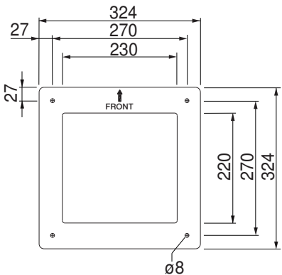
Drilling plan (view X)
