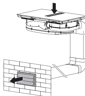
Lateral exhaust air outlet via plinth
