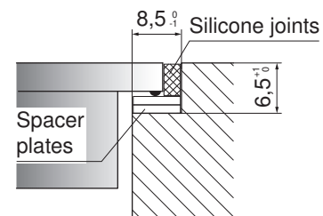
Detail Z
